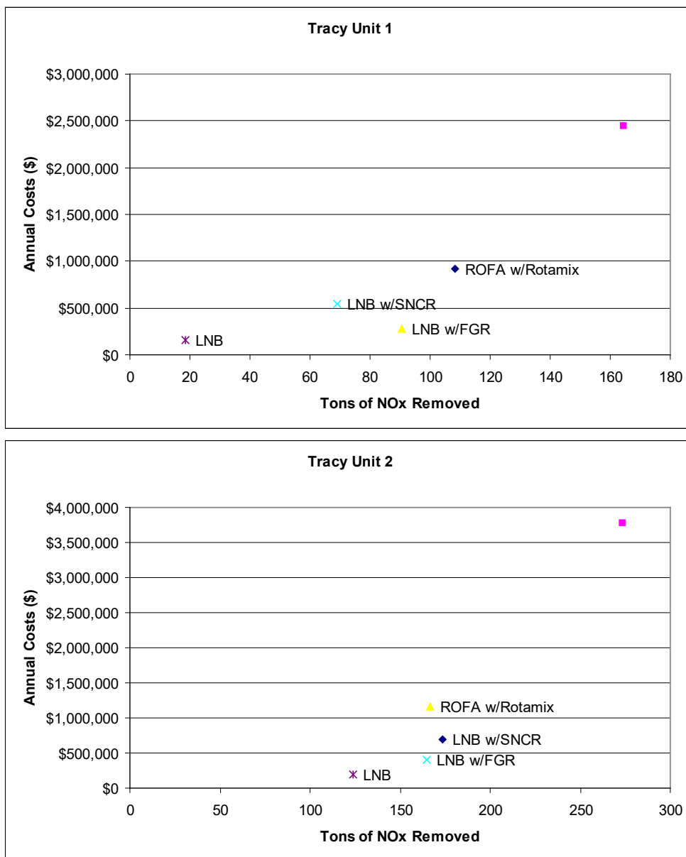
FIGURE 1 LEAST COST ENVELOPE
